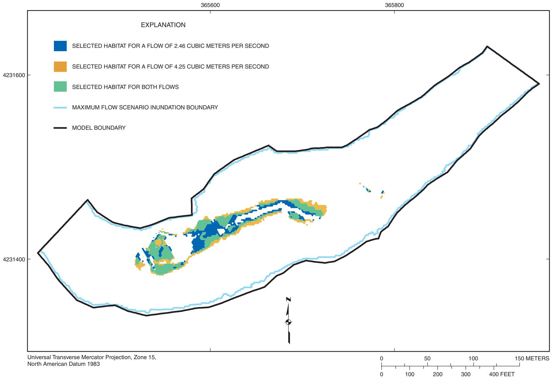
Figure 4-2. Selected habitat area distribution for habitat category 1 (suckermouth minnow) at flows of 2.46 and 4.25 cubic meters per second at Marais des Cygnes River site MDC2.
